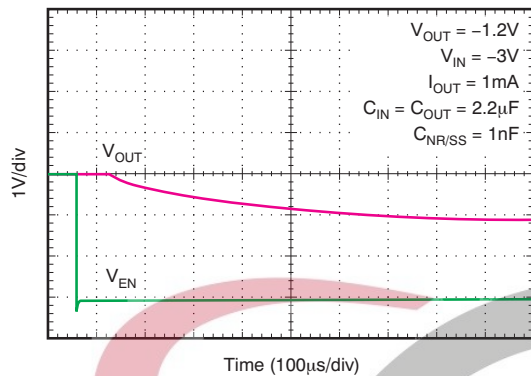
Figure 33. Capacitor-Programmable Soft-Start
